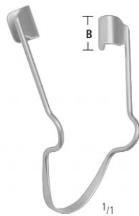
CORCELLE KP 161/05 5,0 cm/ 2" B = 8 mm
